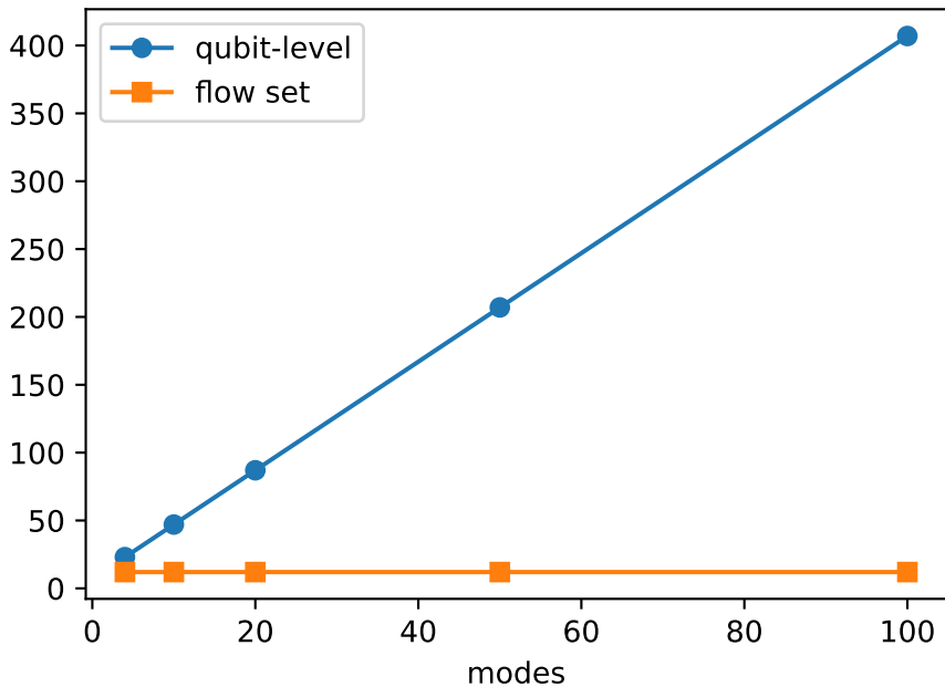
two-qubit depth
