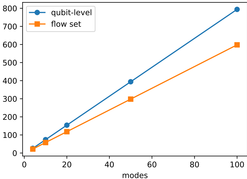
CX count
