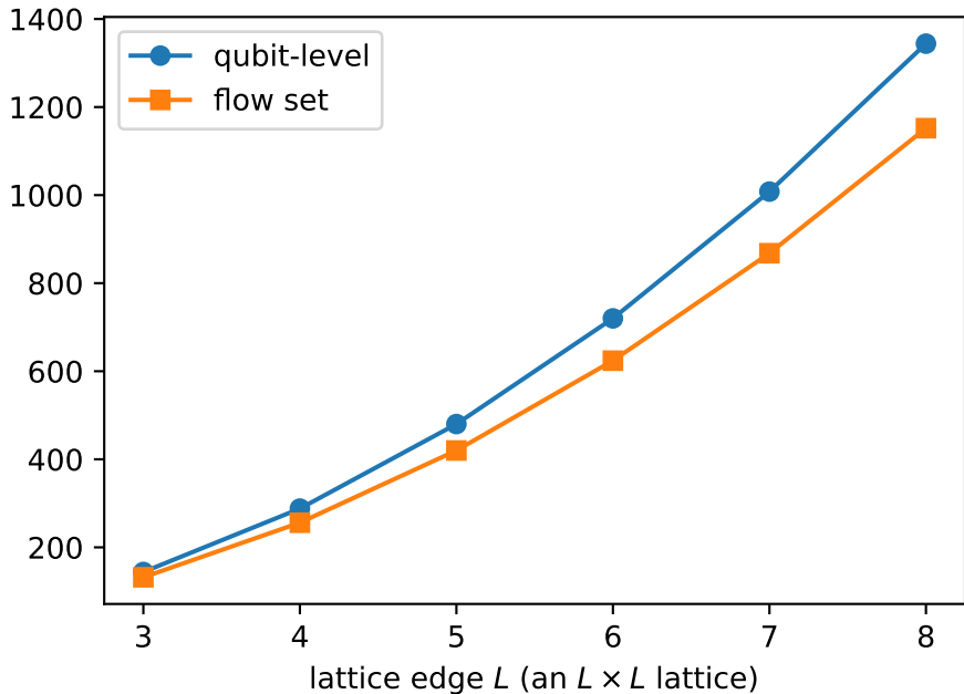
CX count
