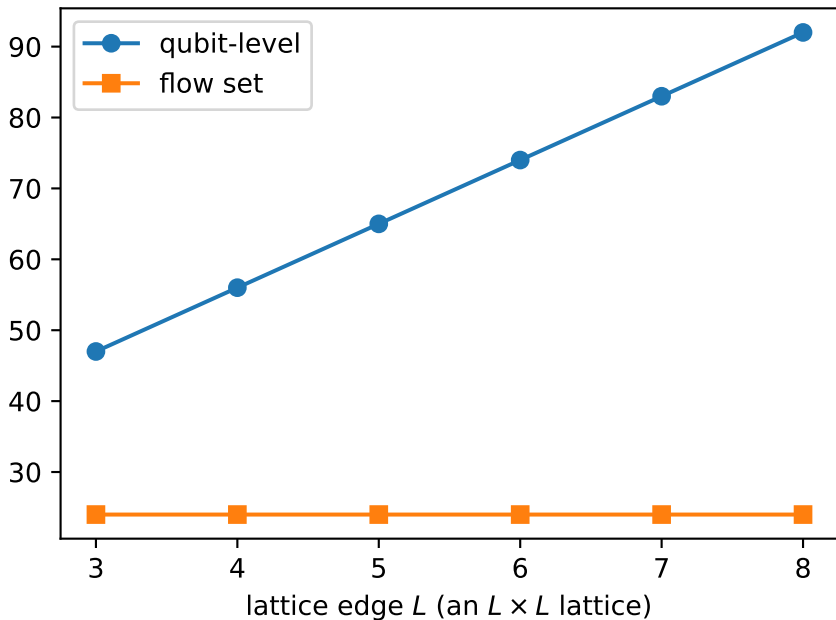
two-qubit depth
